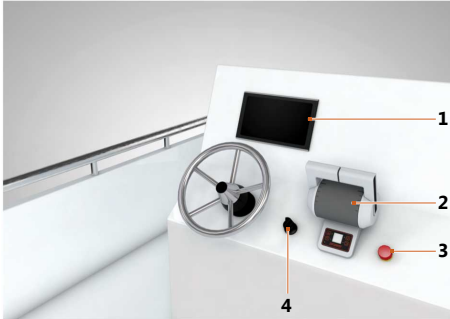
Fig. 1: Controls
