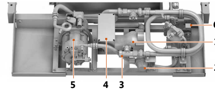
Fig. 11: Battery cooling
