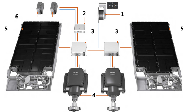
Fig. 2: Components for Deep Blue 40i/80i
