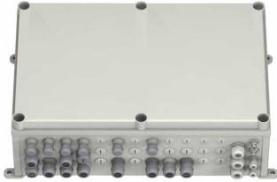
Abb. 59: System Management Unit
