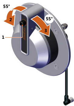
Fig. 42: Operating the remote throttle during forwards/backwards motion
