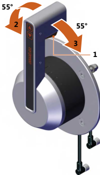
Fig. 43: Operating the remote throttle during forwards/backwards motion
